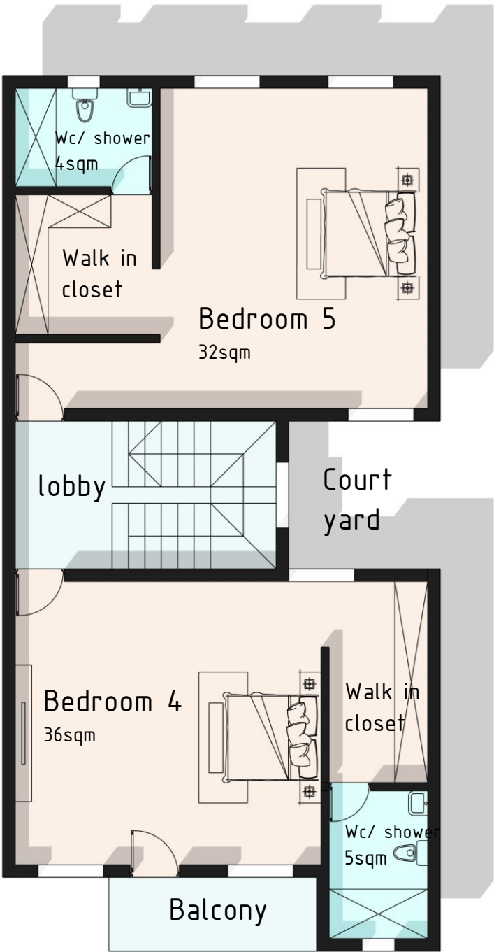
SECOND FLOOR
