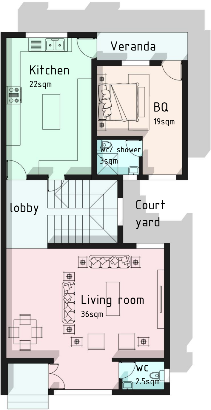
GROUND FLOOR
